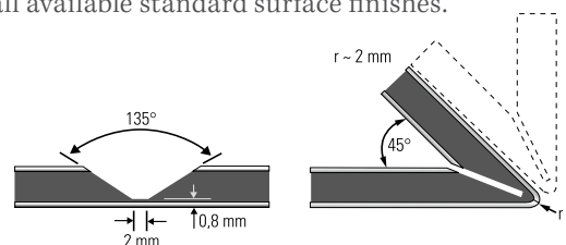
135° V-groove for folds up to 135°
